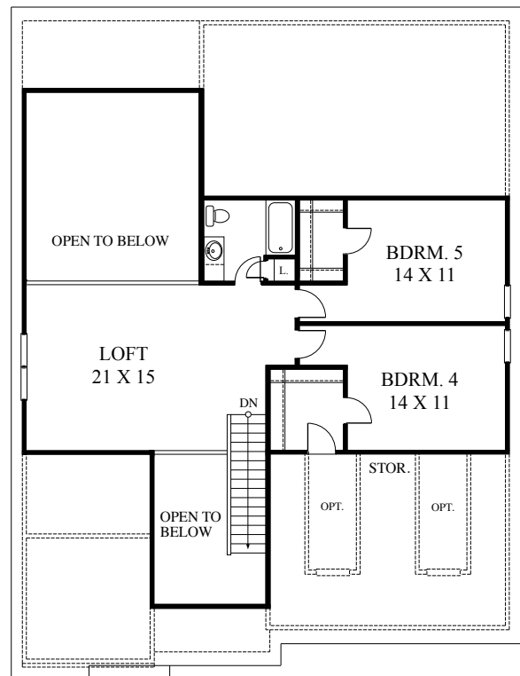
OPT. SECOND FLOOR PLAN
